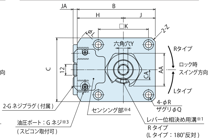
LGM0650-C□-B□ / LGM0750-C□-B□
