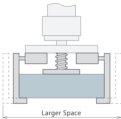
Loading/Lifting Hand with Parallel Hand/Linear Cylinder
