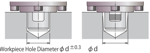
Workpiece Hole Shape: Straight
