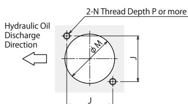
Machining Dimensions of Mounting Hole (Common)
