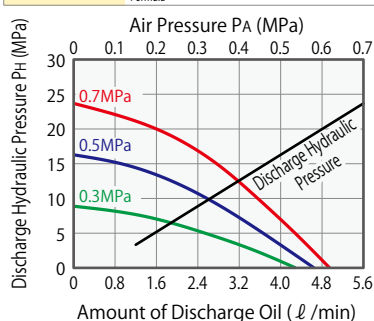
AC6001 Calculation Formula P_H = 37(P_A - 0.06)
