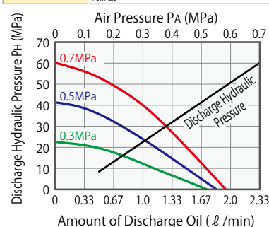
AC8001 Calculation Formula P_H = 94(P_A - 0.06)
