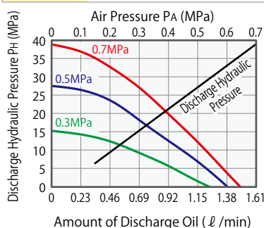
AB7000 Calculation Formula P_H = 59(P_A - 0.04)
