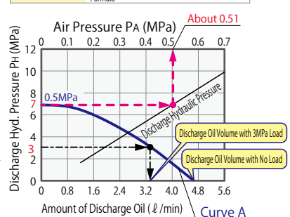
AB4000 Calculation Formula P_H = 15(P_A - 0.04)
