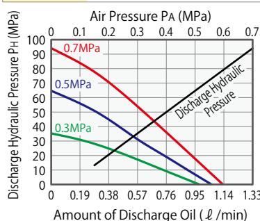
AC9001 Calculation Formula P_H = 147(P_A - 0.06)
