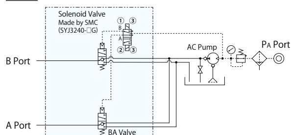
NN Double Action 1 Circuit
