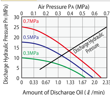
AB6000 Calculation Formula P_H = 38(P_A - 0.04)
