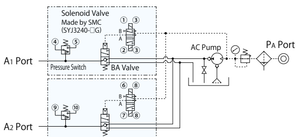
2U Single Action 2 Circuit (With Pressure Switch)
