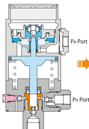
① Initial Position
