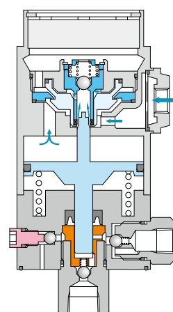
③ Air Supply Switching
