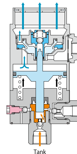
④ Suction Process (Air Vent)
