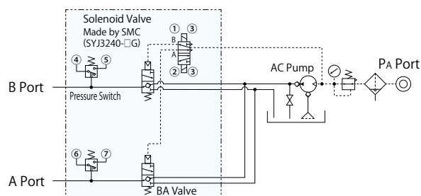
YY Double Action 1 Circuit (With Pressure Switch)
