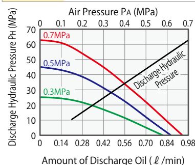
AB8000 Calculation Formula P_H = 95(P_A - 0.04)
