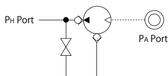
4 Circuit Symbol Blank : Standard
