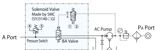
G Single Action 1 Circuit (With Pressure Switch)
