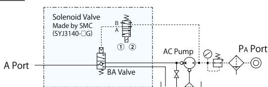
E Single Action 1 Circuit
