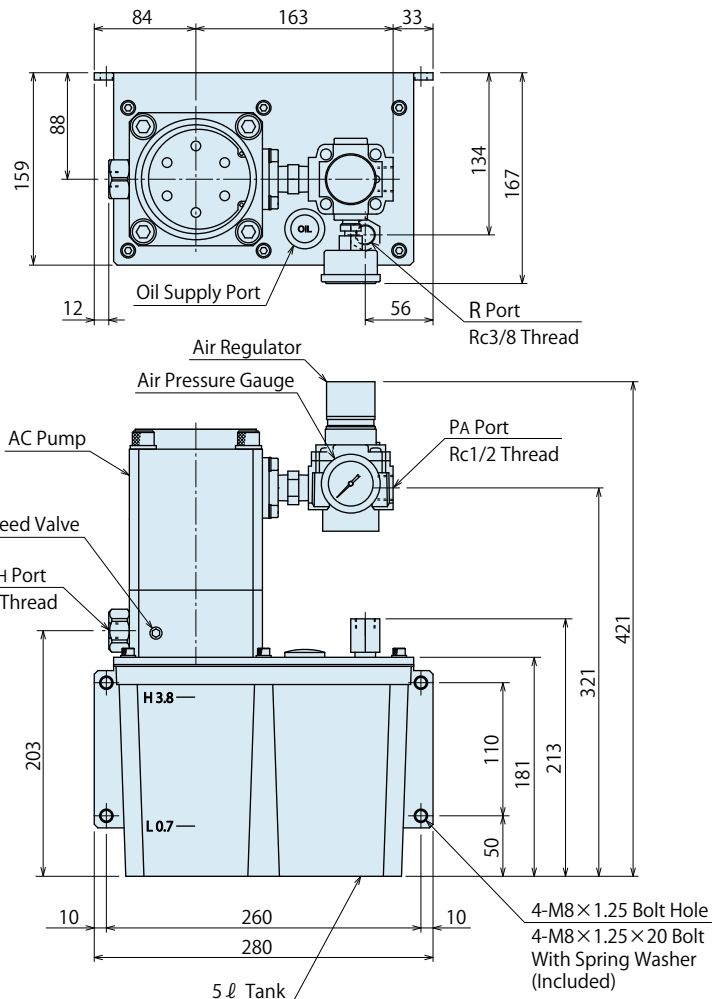
BH Non-Leak Valve Unit
