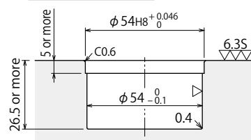
Blind Hole
