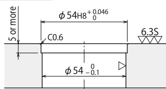
Through Hole
