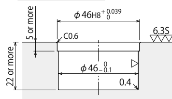
Blind Hole
