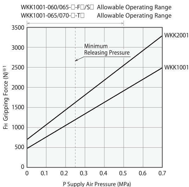
Gripping Force Curve
