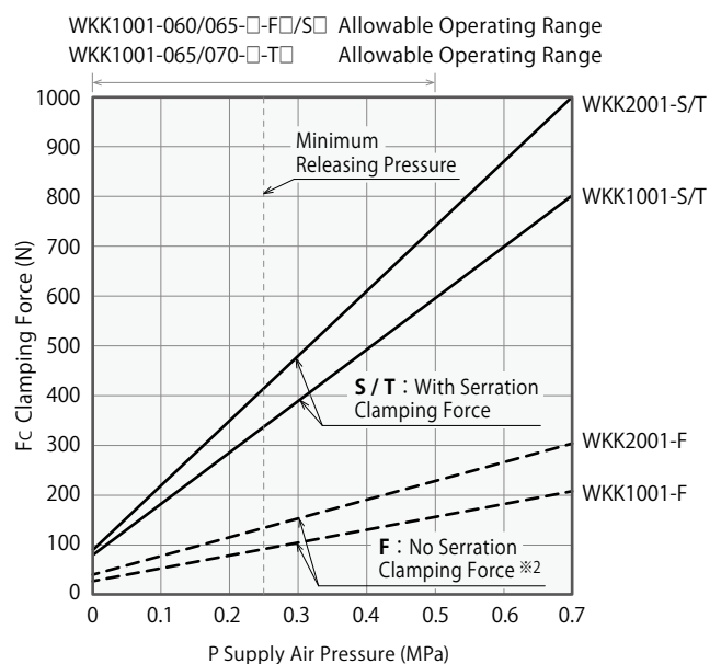
Clamping Force Curve
