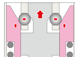
Self-Locking State
