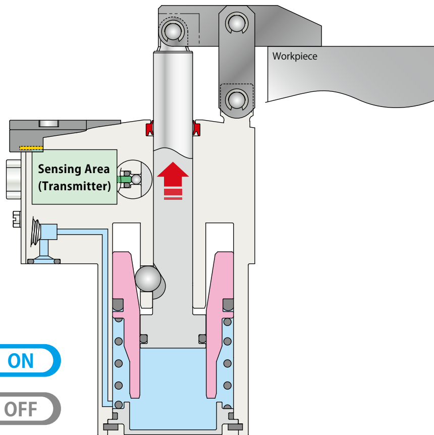
Clamped State
