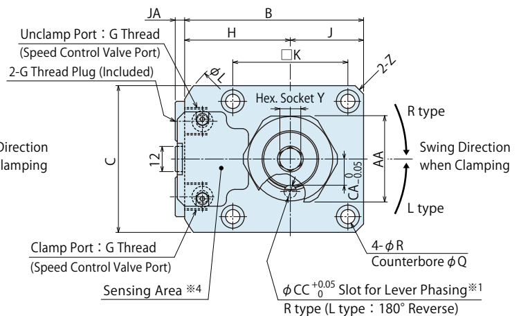
LHM0650-C□-B□ / LHM0750-C□-B□
