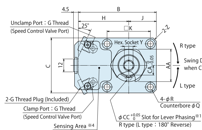
LHM0480-C□-B□ / LHM0550-C□-B□
