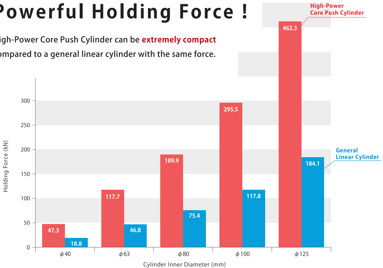
Holding Force Comparison (At Hydraulic Pressure : 15 MPa)
