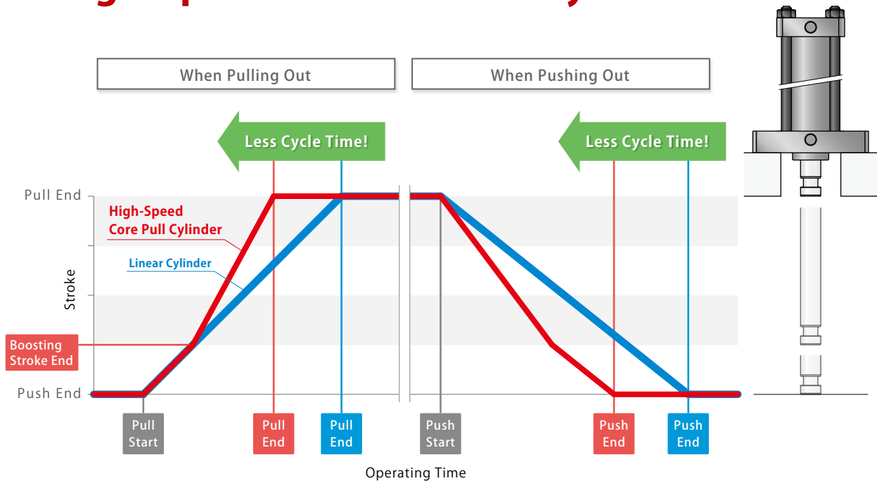
Operating Time Image (Compared to cylinder with the same pulling force.)
