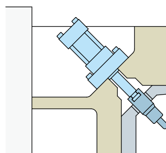
High-Power Core Push Cylinder
