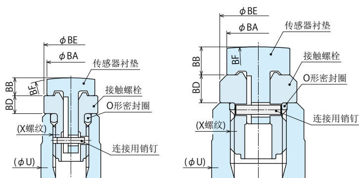
★★剖面 (WNC0603/1003/1603型时)
