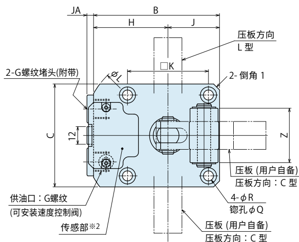
LJM0650-C□-B□ / LJM0750-C□-B□
