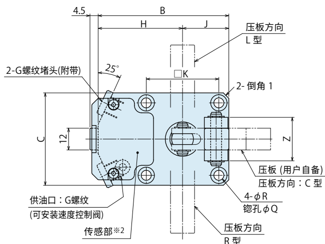
LJM0480-C□-B□ / LJM0550-C□-B□
